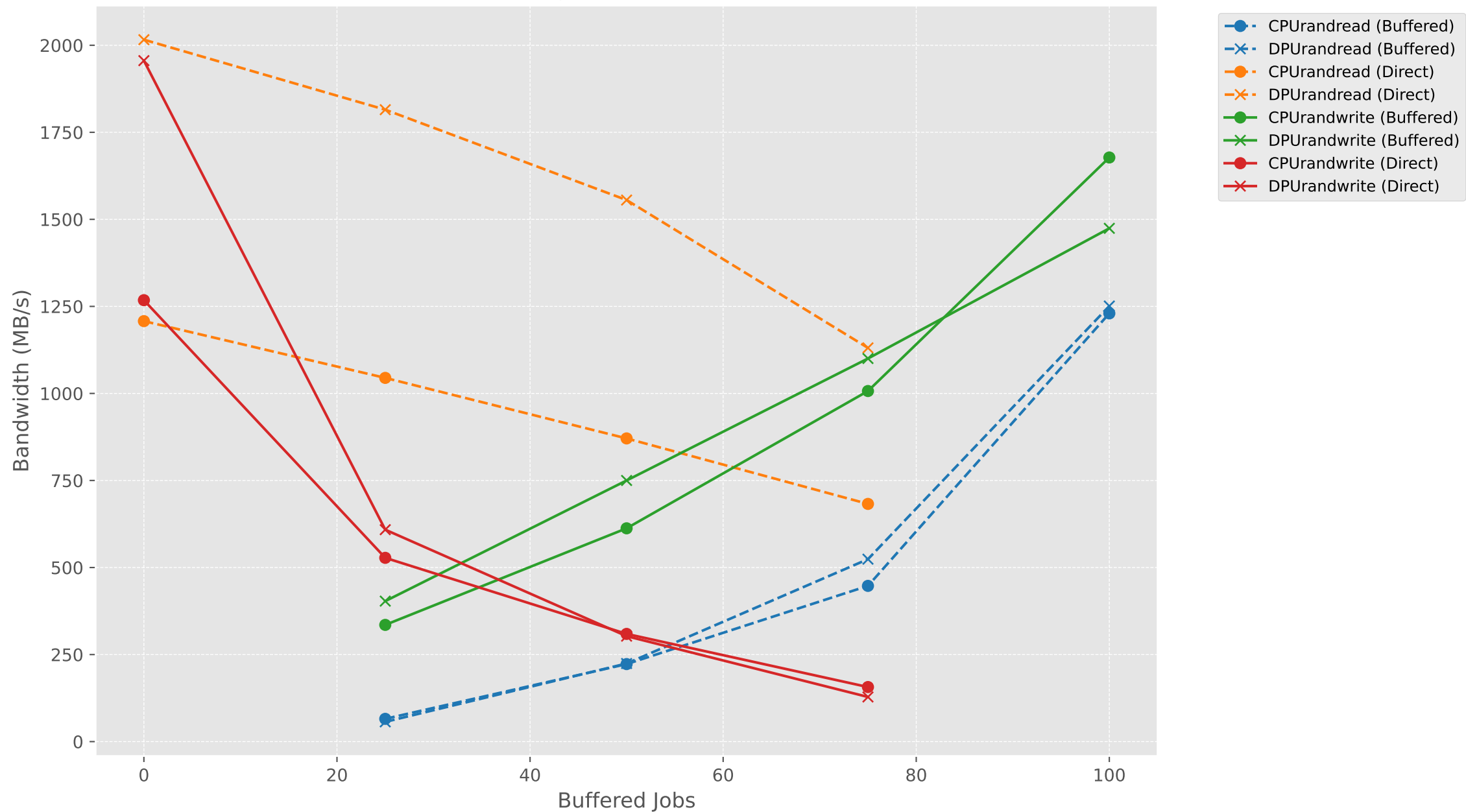
Bandwidth vs Buffered Jobs (mixed) - RAND (CPU vs DPU)
